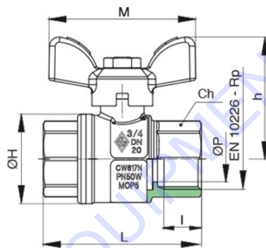
Full bore ball valve, F/F threaded, with aluminum T-handle
