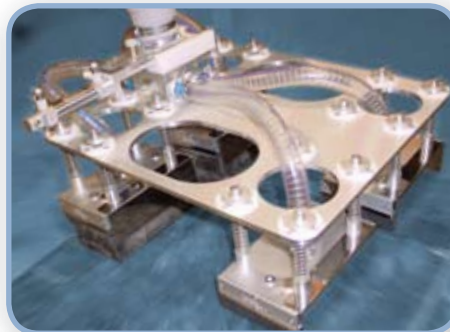
Special-tool with 4 SMS-grippers and external power supply
