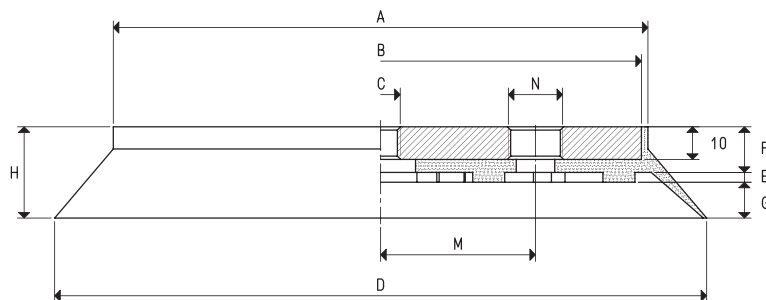
CUPS WITH VULCANISED SUPPORT
