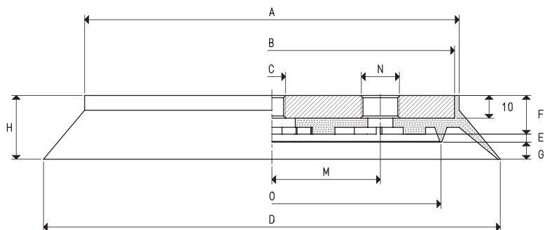
CUPS WITH VULCANISED SUPPORT
