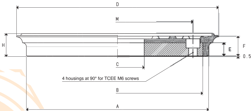
CUP WITH VULCANISED SUPPORT
