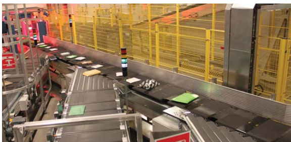
SHOE SORTER
