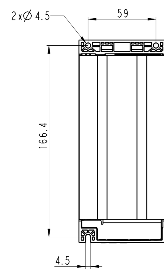
MOUNTING-BASE
