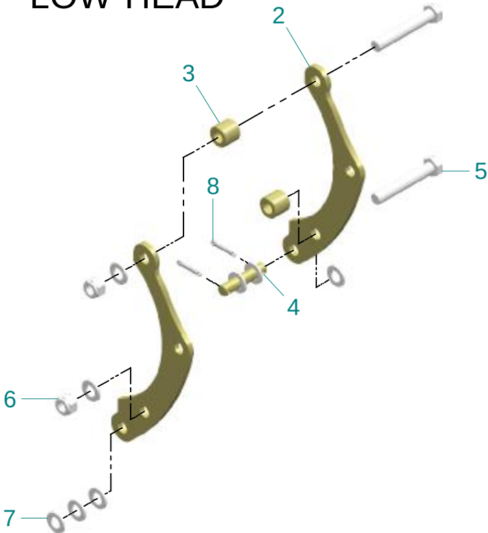
LOW HEAD
