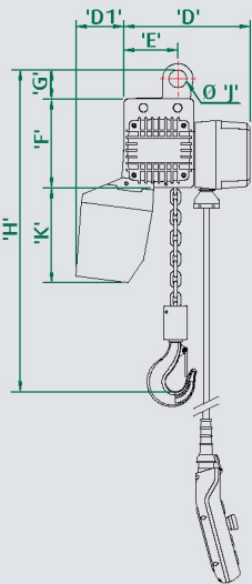
EYE SUSPENSION
