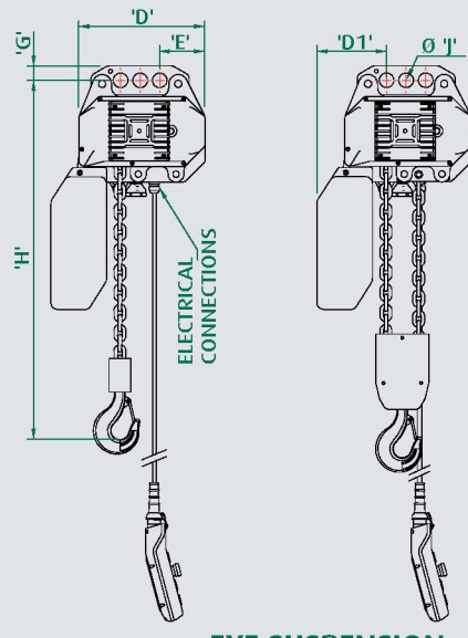
EYE SUSPENSION
