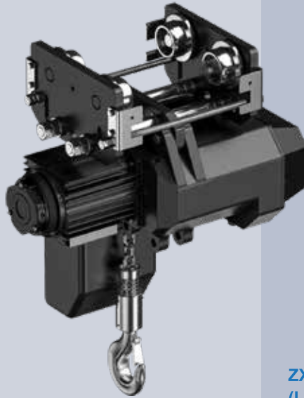
LX CHAIN HOIST >>> WITH PUSH TROLLEY (Standard Headroom) Capacity of 0.5 Tons to 5 Tons Lifting height 6 Meter
