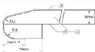
WORKTOP PROFILE TYPE 9
