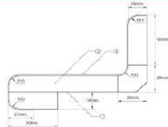
WORKTOP PROFILE TYPE 10
