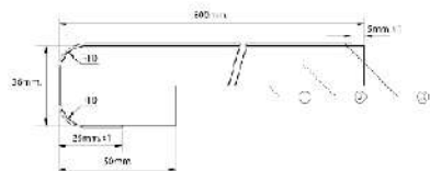
WORKTOP PROFILE TYPE 5
