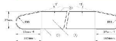
WORKTOP PROFILE TYPE 4
