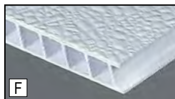
F. 0.4-inch FiberCorr Liner Ceiling, 2-feet x 4-feet textured FRP panel with no substrate backer.
