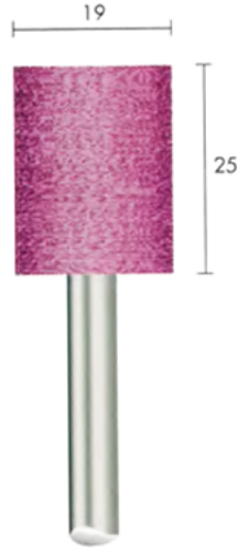
W-205 (19x25mm.)
