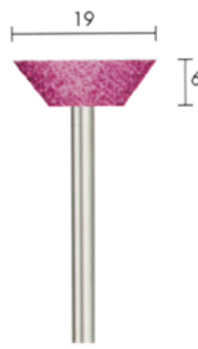
R-1906 (19x6mm.)
