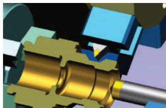
Turning
