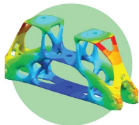
Topology Design
