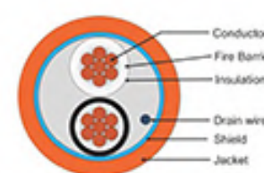
FRC 1 Pair cable, Shielded
