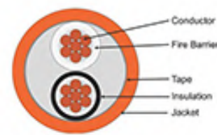
FRC 1 Pair cable, Unshielded
