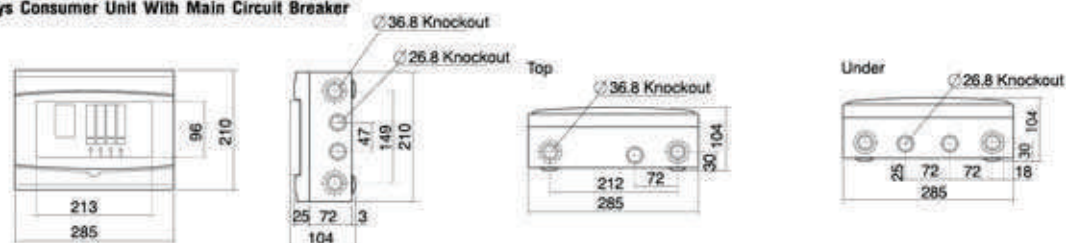
Figure 7 - 4, 6 Ways Consumer Unit With Main Circuit Breaker
