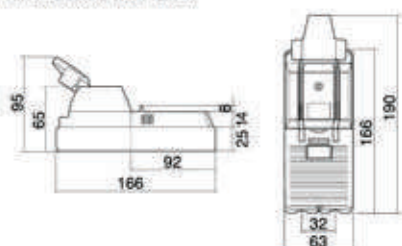
Figure 18 - 2P Knife Switch With Cover
