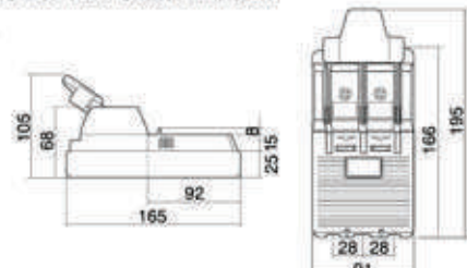
Figure 19 - 3P Knife Switch With Cover
