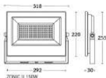
ZONIC II 150W
