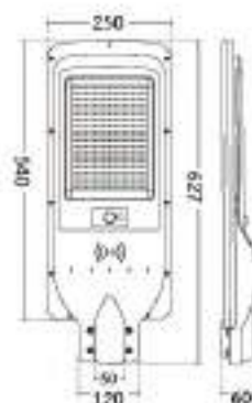
OSLO 150W
