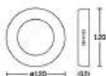
WINE-O 6W
