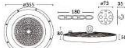
WOLF 200W/6500K
