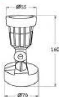
LUNAR-P 5W/3000K
