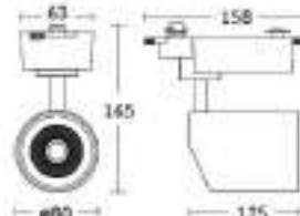
OSCAR 25W
