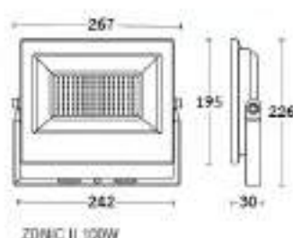
ZONIC II 100W
