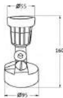
LUNAR-2P 2x5W/3000K
