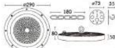
WOLF 150W/6500K
