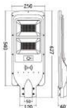
OSLO 200W
