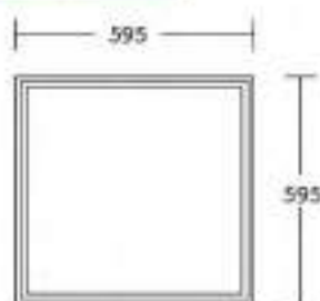
PANEL48W / 60x60
