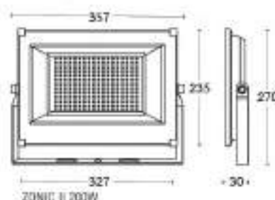
ZONIC II 200W
