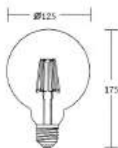
VINTAGE-G/G 8W/2700K
