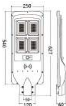
OSLO 120W
