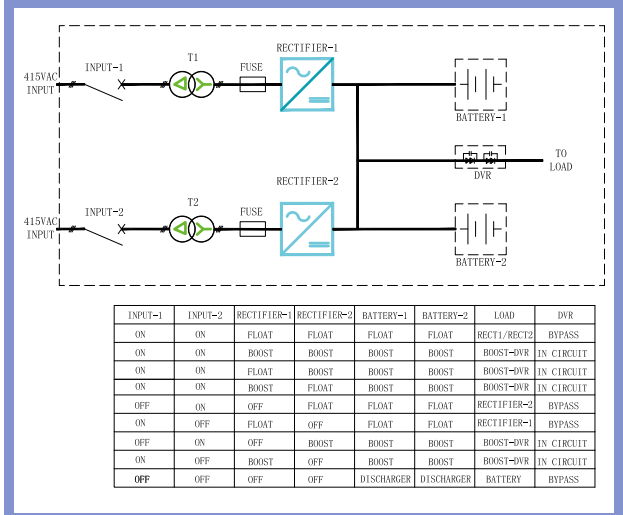
Redundant Float Cum Boost Charger with Diode Dropper-Single Load-Dual Battery Bank
