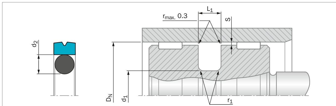
Figure 115: Installation Drawing
