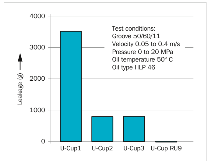
Figure 57: Leakage performance dependent on U-Cup type
