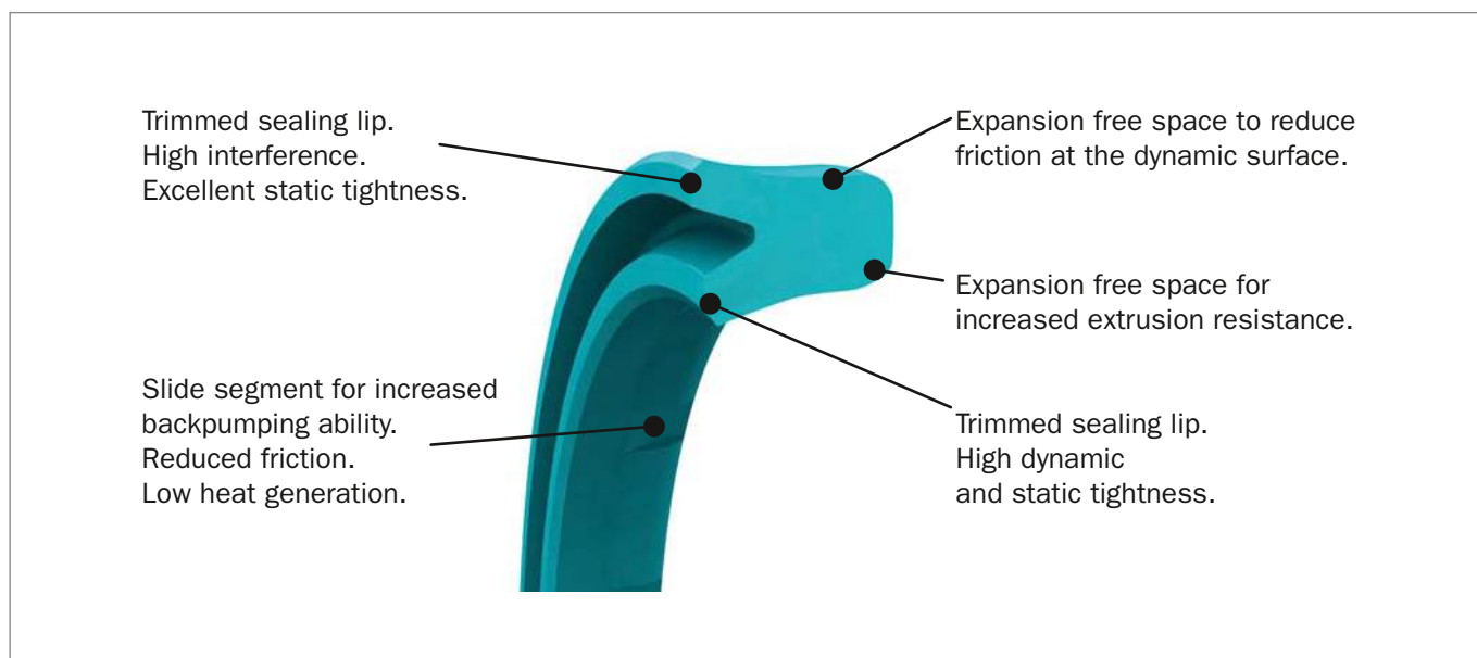
Figure 53: Zurcon® U-Cup RU9 design features
