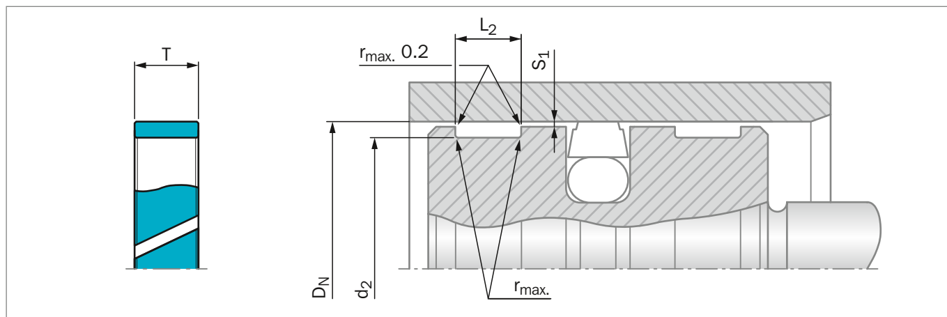
Figure 205: Piston guide
