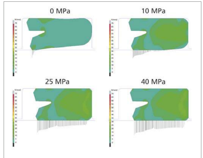
Figure 56: How the Zurcon® U-Cup RU9 performs underpressure
