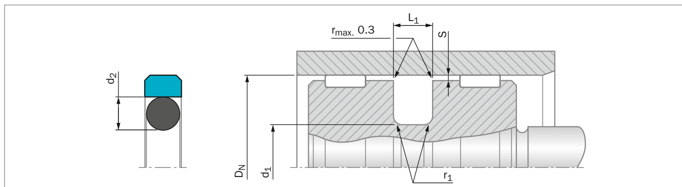
Figure 109: Installation Drawing
