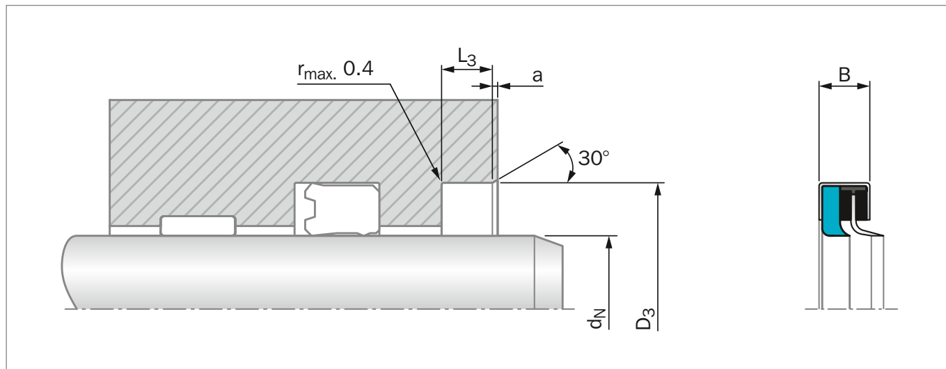
Figure 199: Installation Drawing
