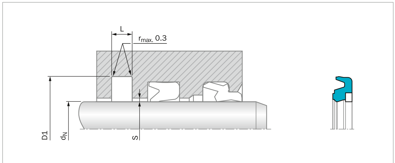
Figure 65: Installation Drawing
