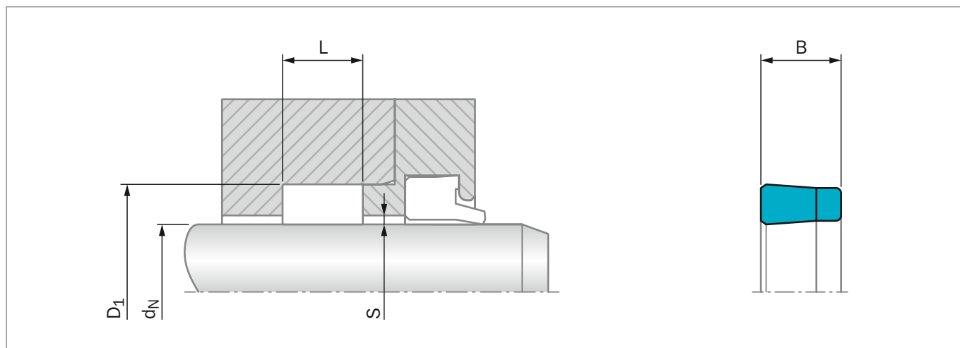
Figure 40: Installation Drawing
