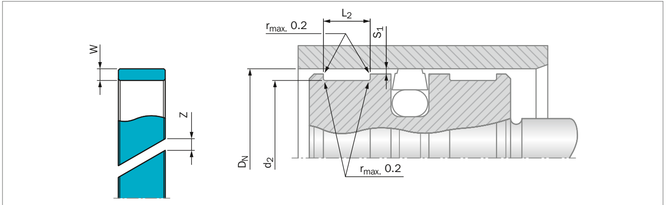
Figure 211: Installation Drawing
