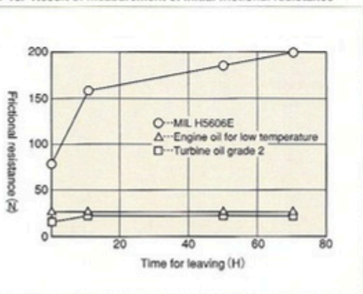
<Fig. 1-13> Result of measurement of initial frictional resistance
