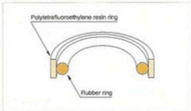
<Fig. A-5> Example of combined seal
