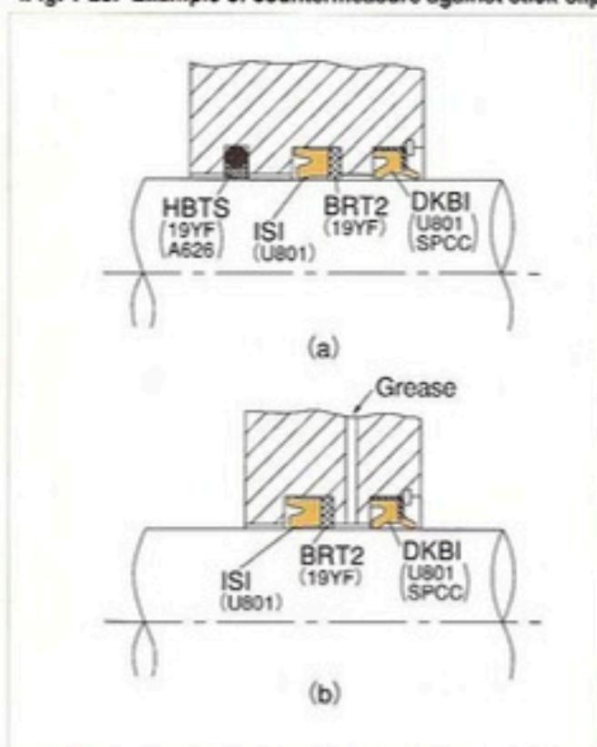
<Fig. 1-23> Example of countermeasure against stick-slip
