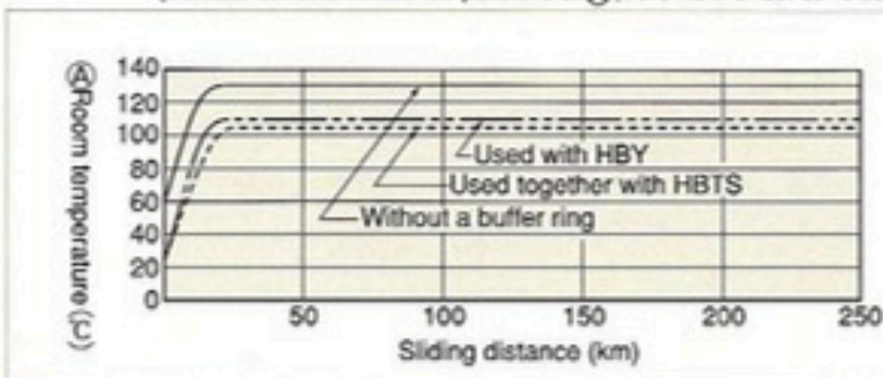
<Fig. 1-14> An example of measurement of temperature at sliding area (For test conditions and temperature at (A), refer to the test condition.)
