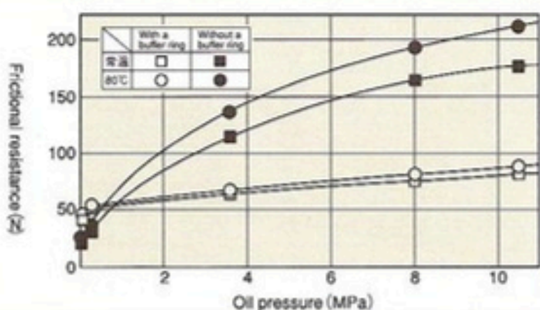
<Fig. 1-15> Relation between hydraulic pressure and frictional resistance
