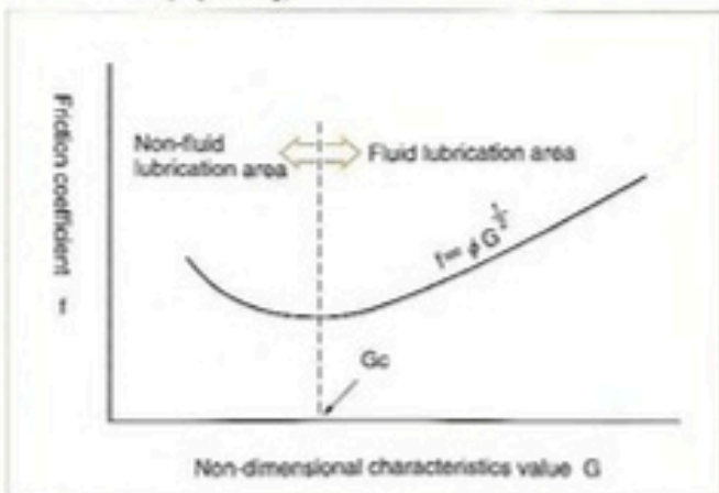
<Figure A-8> Example of non-dimensional characteristics graph (U packing)
