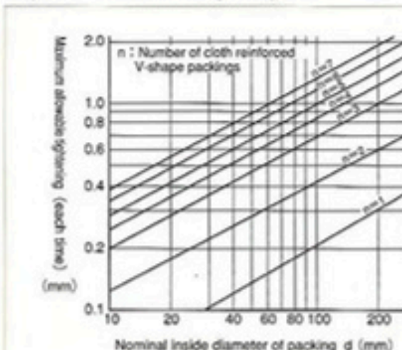
<Fig. G-28> Max. allowable tightening
