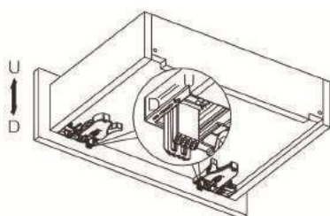
Height adjustment 0~+3mm
