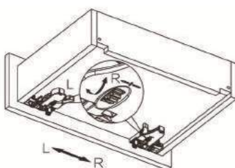
✱ Side adjustment \pm 1.5\text{mm}
