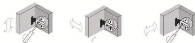
Three-dimensional adjustment
