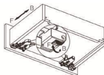
Depth (In and Out) adjustment 0~+3mm
