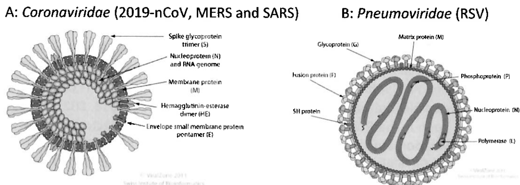
Figure 1: Icon representation of the enveloped and spherical viral particles (Viralzone).
