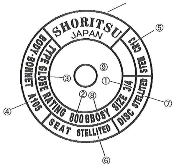
Figure 8.1 Example for globe valve (Class 800, NPS 3/4")
