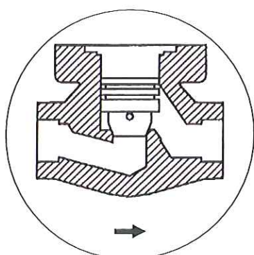
Cross section of valve body
