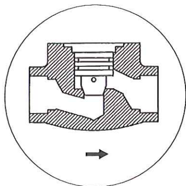
Figure 1.6 Typical Examples for Class 800 Check Valve
