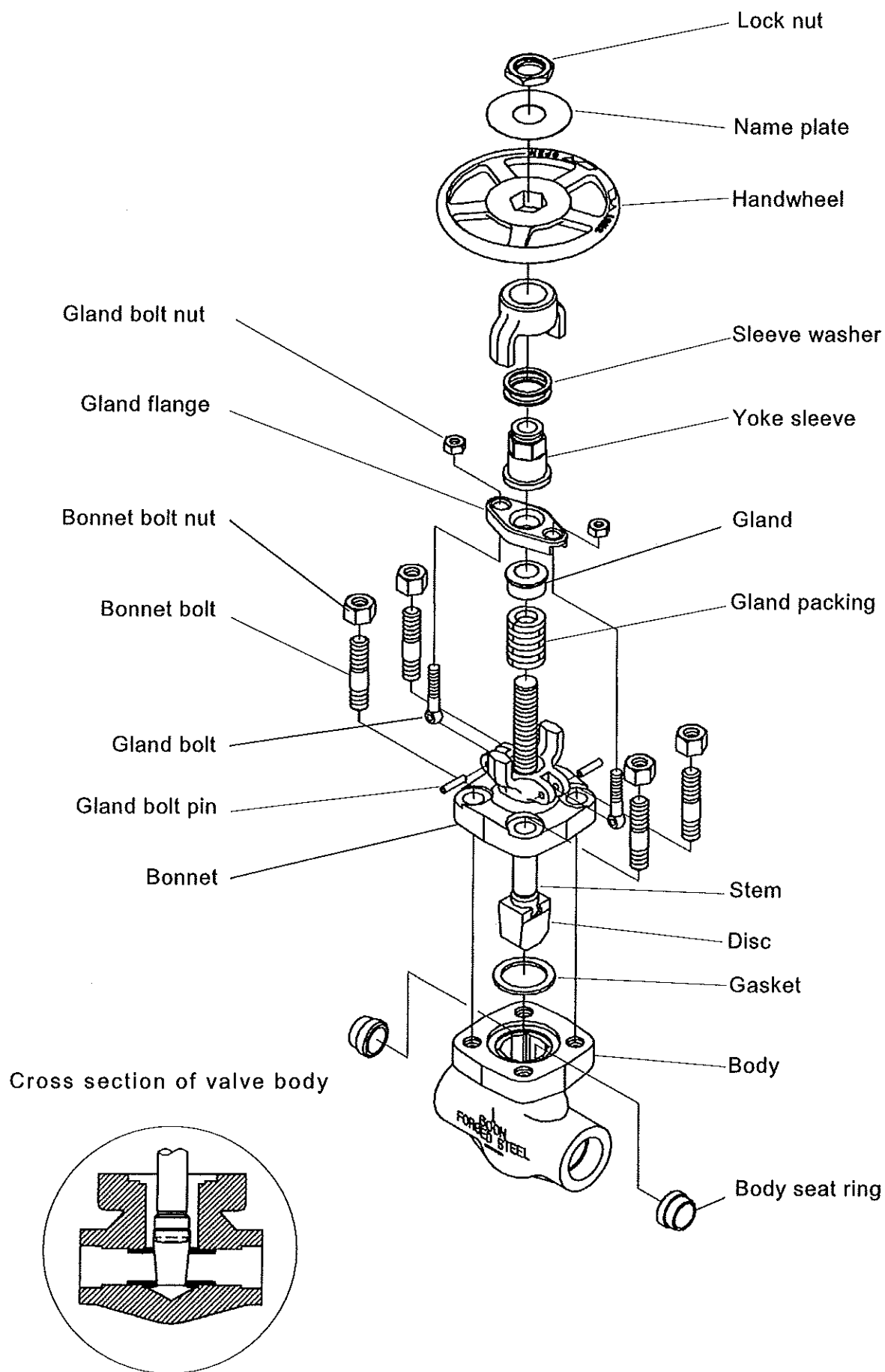
Figure 1.1 Typical Examples for Class 600 Gate Valve
