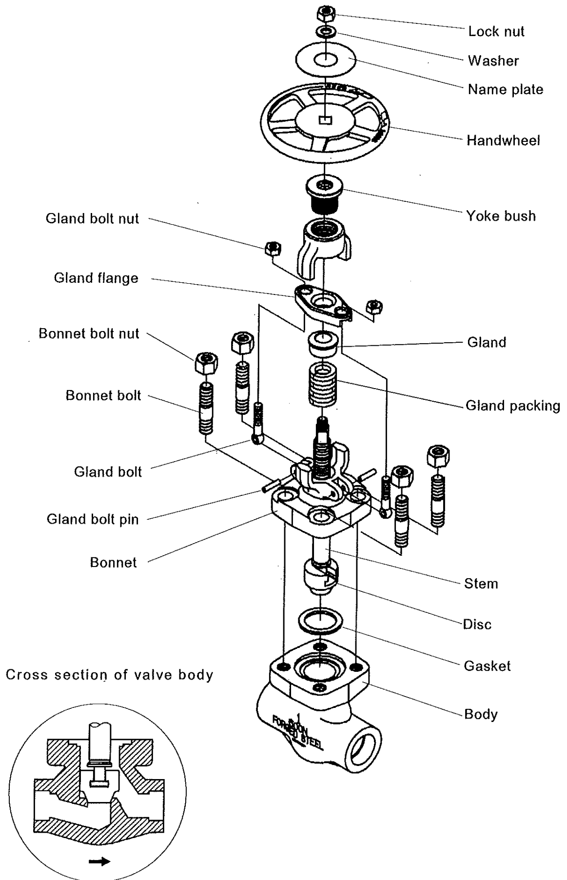
Figure 1.3 Typical Examples for Class 600 Globe Valve
