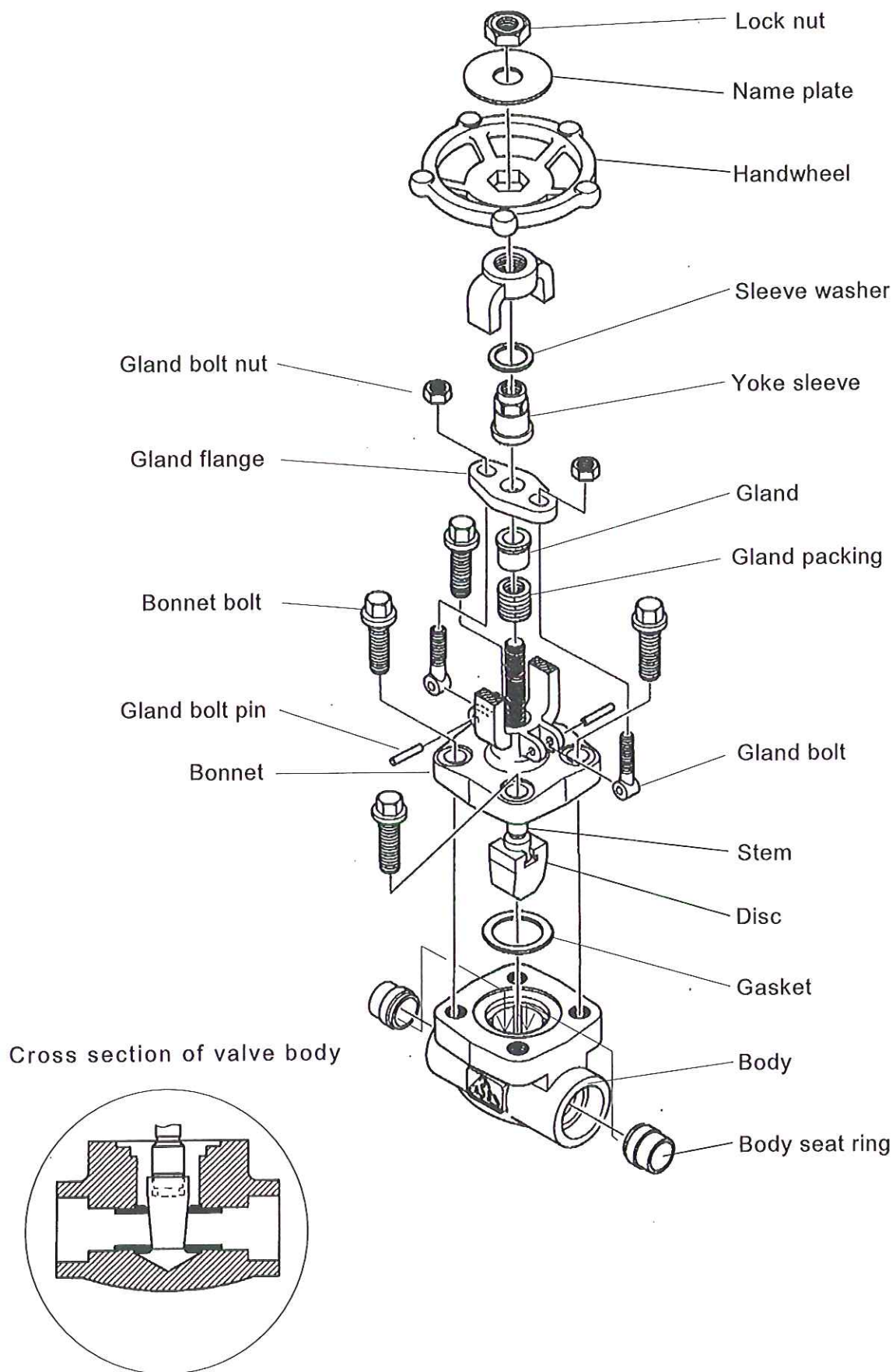
Figure 1.2 Typical Examples for Class 800 Gate Valve
