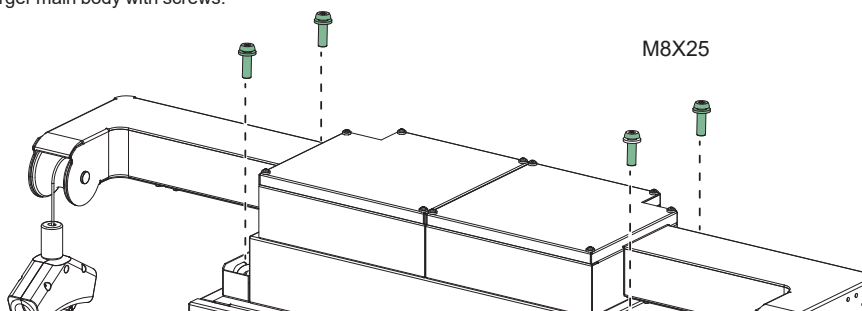
Fixing the adapter plate and the charger main body
