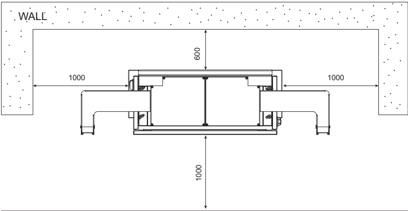
Floor Standing Service Clearances
