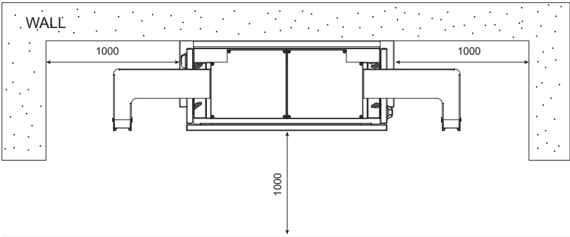
Wall Mounted Service Clearances
