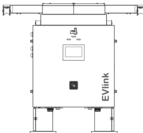
Effect drawing of cable management system installation
