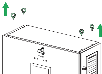
Removing the hoisting rings
