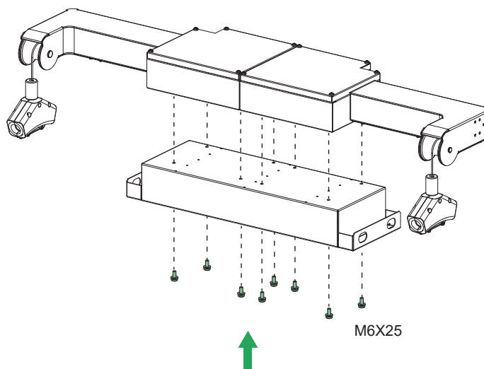
Installing the Cable Management System on the adapter plat
