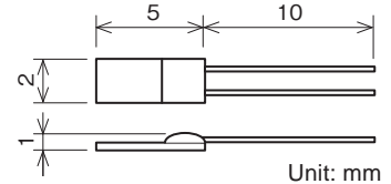
External dimensions
