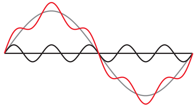
The total current as the sum of the fundamental and 5 th harmonics
