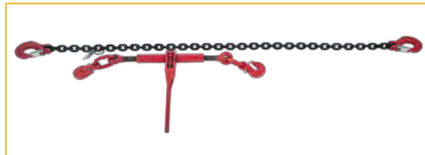
Lashing chain 2-part
