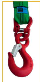
TLX Round sling with on each leg a PES-TLX sleeve
