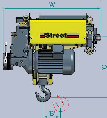
ZX08 Single Girder Hoist
