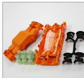
Ordering Code: 9-0904-00 Gel-Filled IP68 connector for through wiring. For cable diameter 6.5 - 12mm
