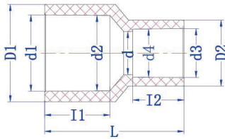
异径直接 REDUCER COUPLING (S×S) DIN
