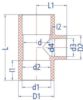
异径三通 REDUCER TEE (S×S×S) DIN
