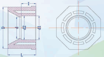
补芯 REDUCER BUSHING (S×S) ANSI
