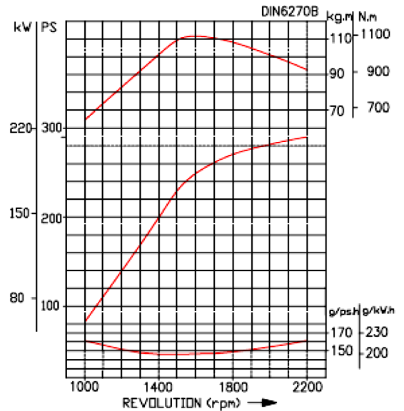
© PERFORMANCE CURVE
