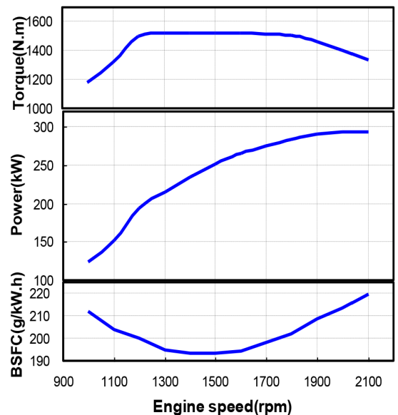
© PERFORMANCE CURVE
