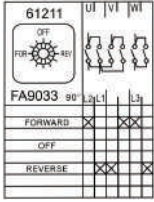
Forward Reverse Switches
