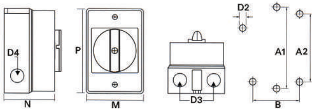
Dimension IP65 plastic box
