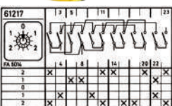
Reversing 2 Speed Switches
