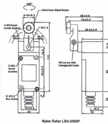
Nylon Roller LSN-5000P
