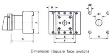
Dimension (Square face switch)
