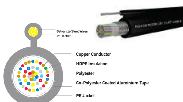
FIG-8 OUTDOOR CAT 3 UTP Cable
