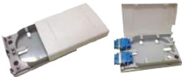
UF-1002 2 Port Home Fiber Termination Box (W140* H90* D25 mm. )
