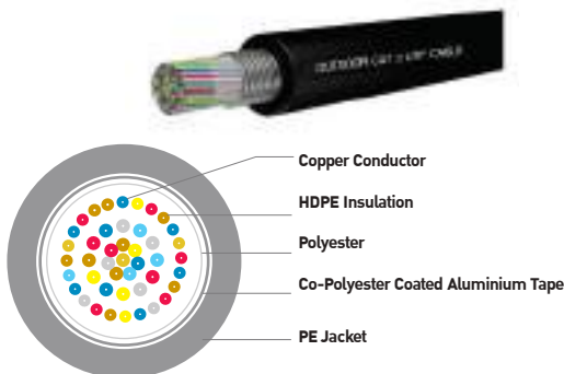
OUTDOOR CAT 3 UTP Cable
