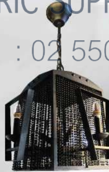
F 49-3009-8 SIZE : D:550x550 mm H:2450 mm LAMP :E14x8 COLOR :SBK MATERIAL : STEEL
