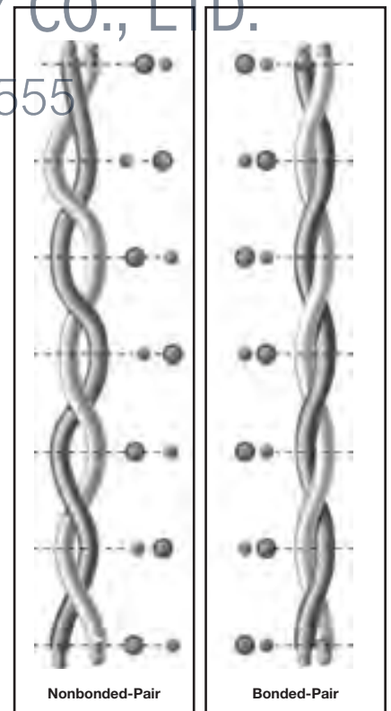
Nonbonded pairs can lose the uniformity of twist that is essential to consistent electrical performance.
