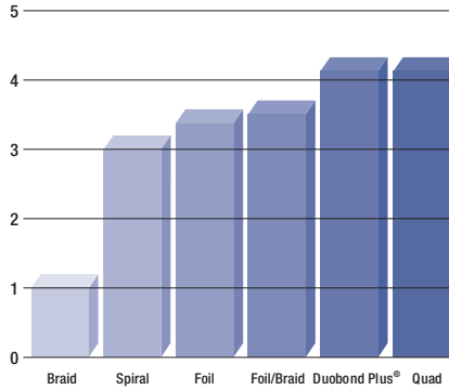
Shield Performance Comparison Chart
