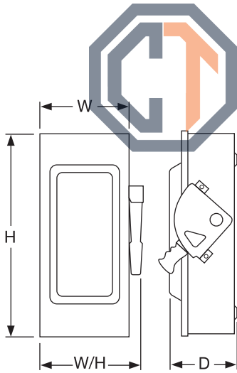
Typical NEMA 1
