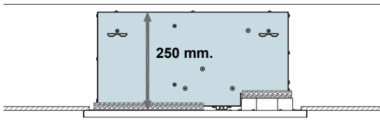
Model 12,000-24,000 Btu/Hr.
