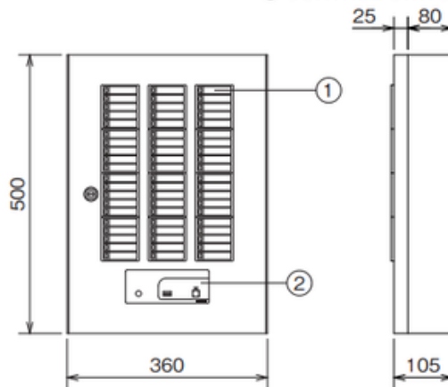
② CONTROL SWITCH PART
