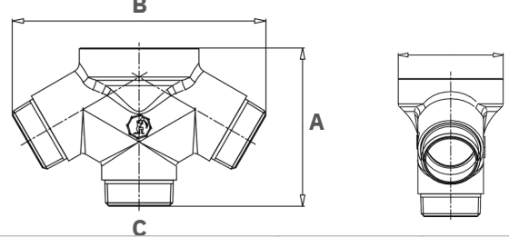
A97 – NPT INLET (F) x THREE NPT OR HOSE THREAD OUTLETS (M)
