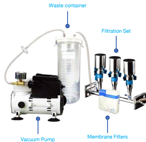
Vacuum Pump Filtration System
