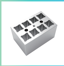
TC0401005-45 8-12.5x12.5x32mm (used in cuvette)
