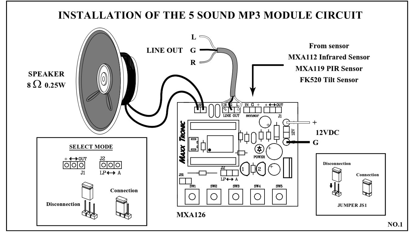
CIRCUIT DIAGRAM
