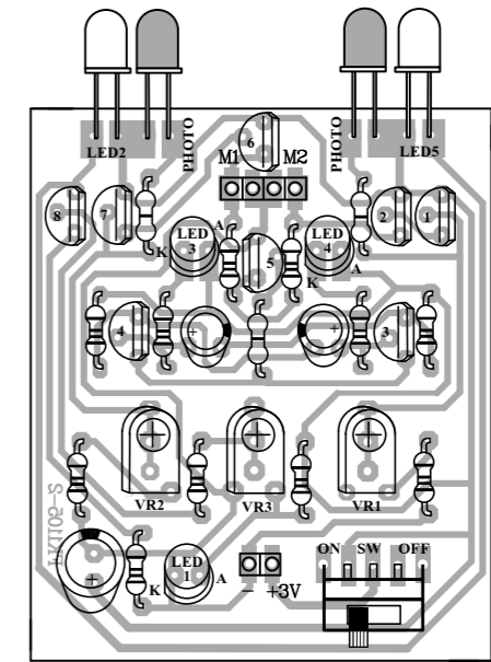
Circuit Assembling
