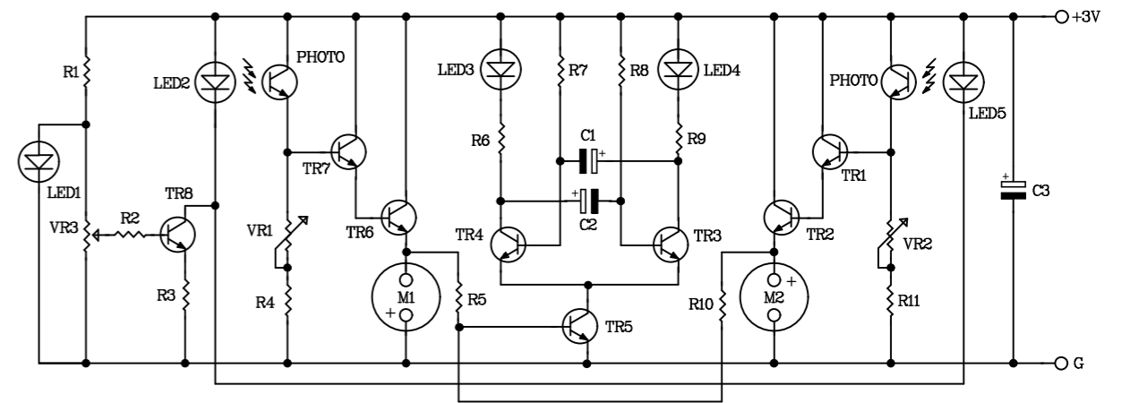
Figure 1. TACON Line Follow Robot Circuit
