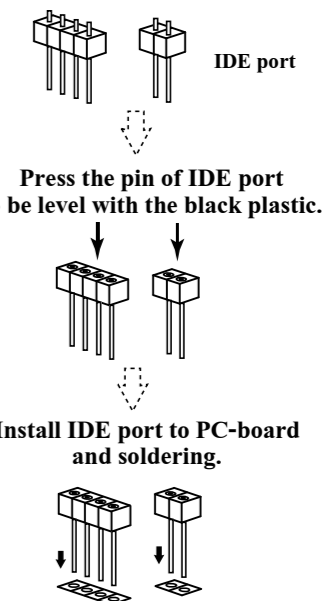
Figure 4. IDE Port Assembling To The Circuit Board.
