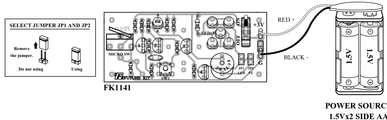
Figure 2. Circuit Assembling
