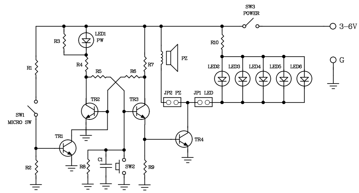
Figure 1. Checkpoint Circuit
