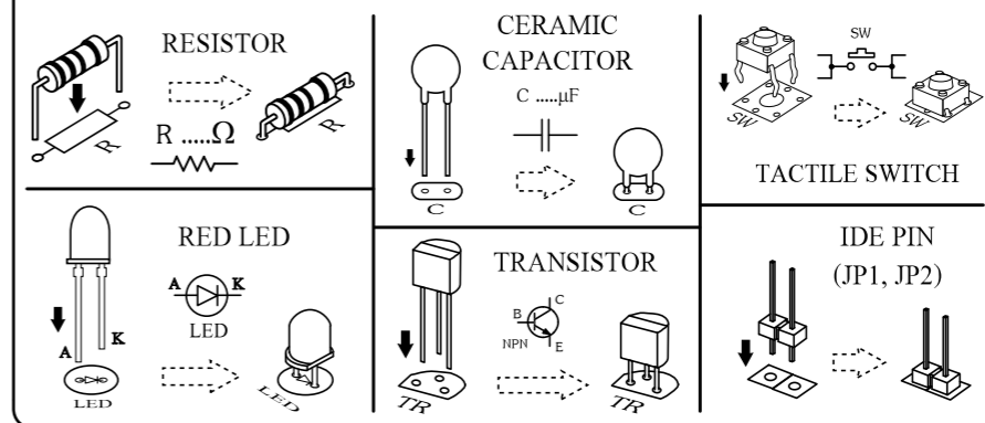
Figure 3. Components Installing
