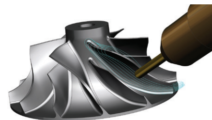
Blade finishing.
