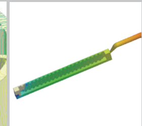
Short Shot
