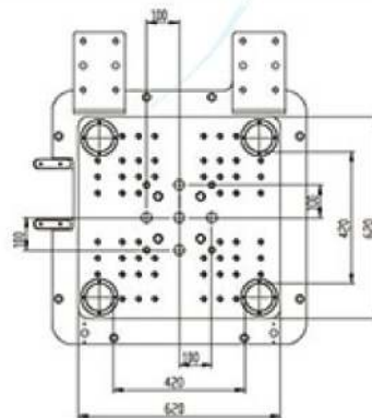
Stationary Platen
