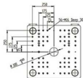
Moveable Platen
