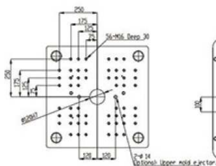
Moveable Platen
