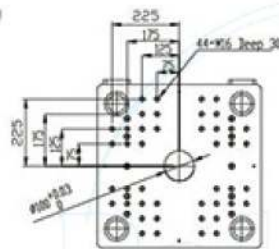
Moveable Platen
