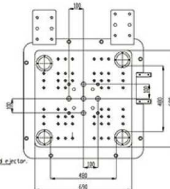
Stationary Platen
