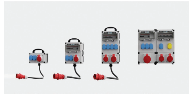
VARIABOX-S Mobil 130 x 230 mm VARIABOX-M Mobil 260 x 230 mm VARIABOX-L Mobil 390 x 230 mm VARIABOX-L DUO 520 x 230 mm
