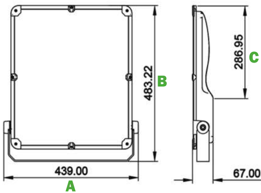
DIMENSION (Unit: mm.)
