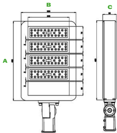
DIMENSION (Unit: mm.)
